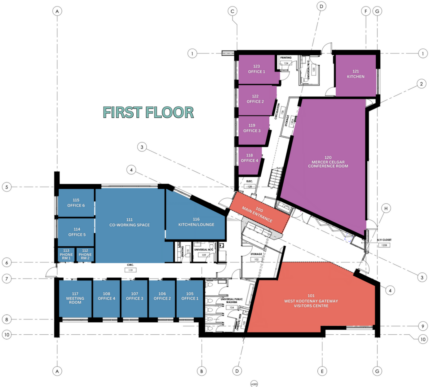
1 OVERALL MAIN FLOOR PLAN 1:75
